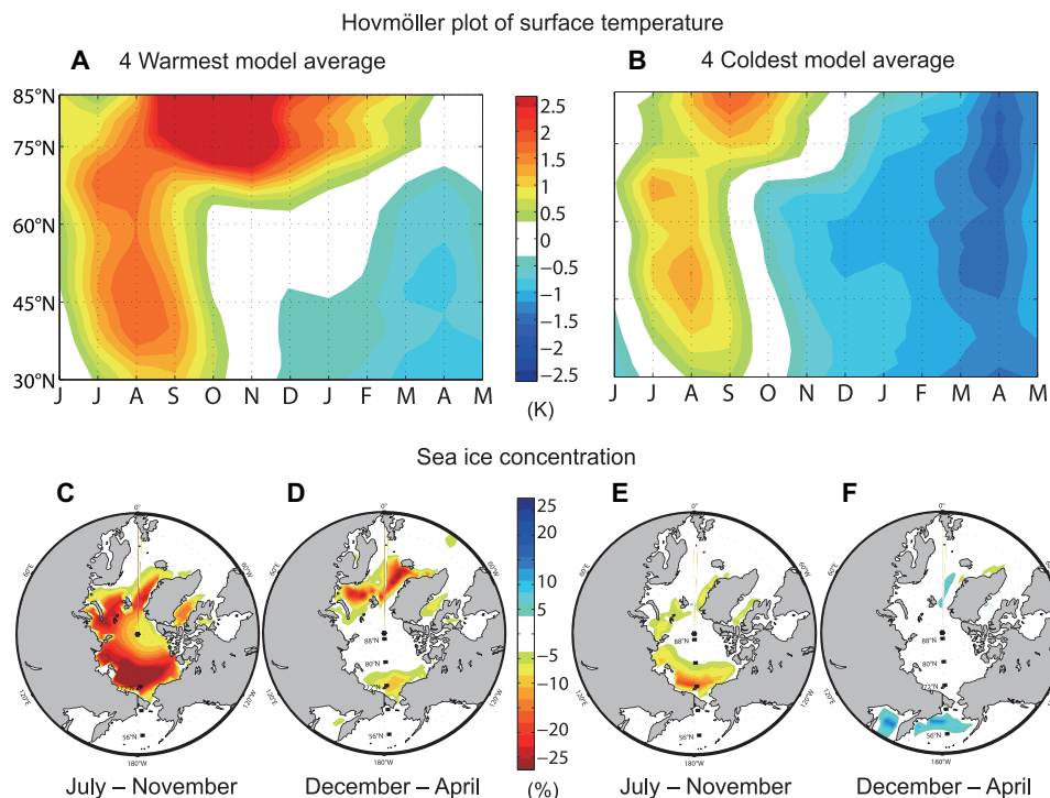
Fig. 2. Surface temperature and Arctic sea ice responses. (A and B) Zonally averaged, latitude-time Hovmöller plots of surface temperature anomalies in (A) the four warmest models and (B) the four coldest models. The abscissa is time (months) and the ordinate is latitude. Arctic sea ice concentration (SIC; %) anomalies in (C and D) the four warmest models and (E and F) the four coldest models, averaged in (C and E) July to November and (D and F) December to April.
